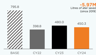
Annual Consumption Intensity (L/m 2 )
